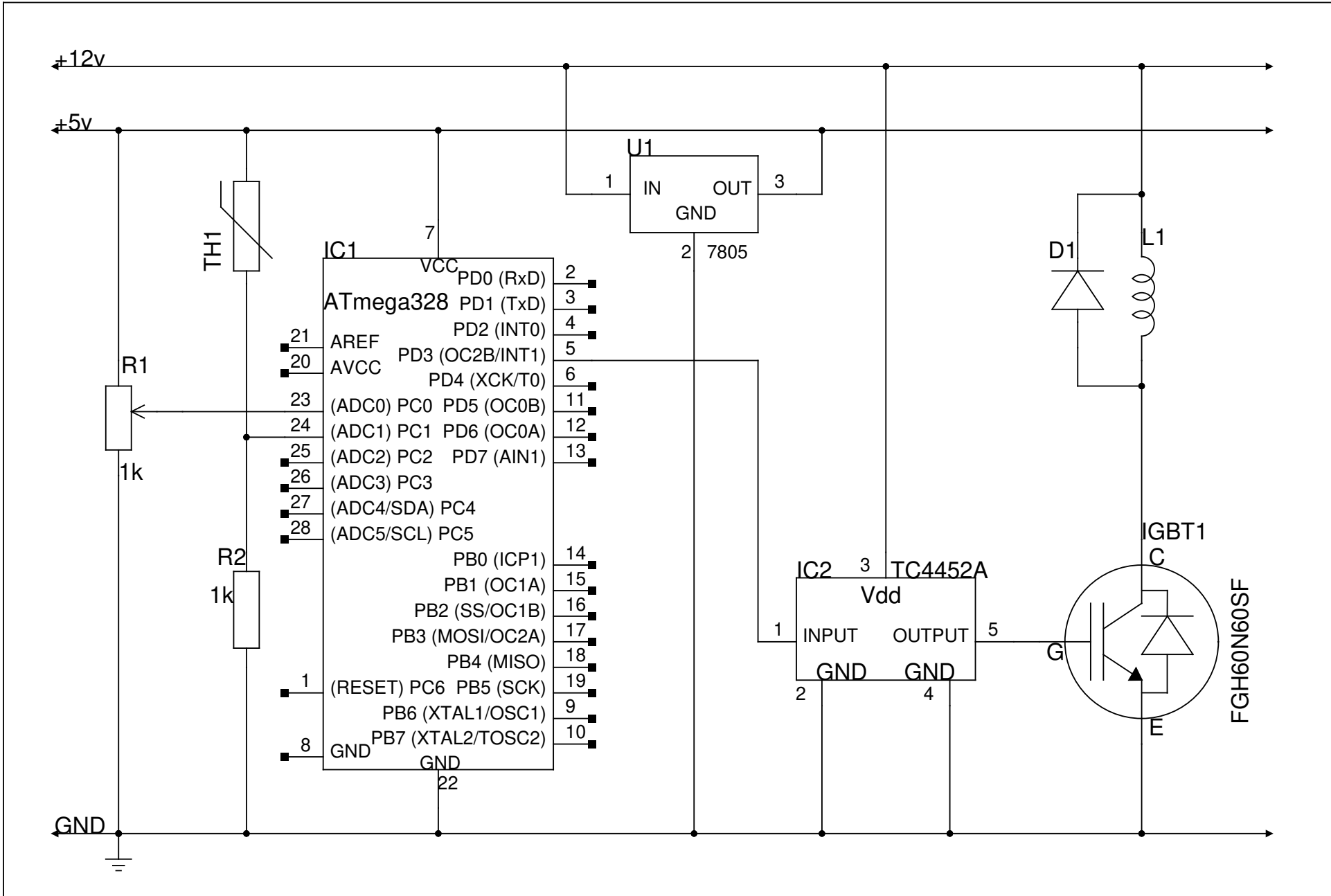
TITLE: Solenoid test | AUTHOR: Graham North | CREATED: 25-Jan-2020
