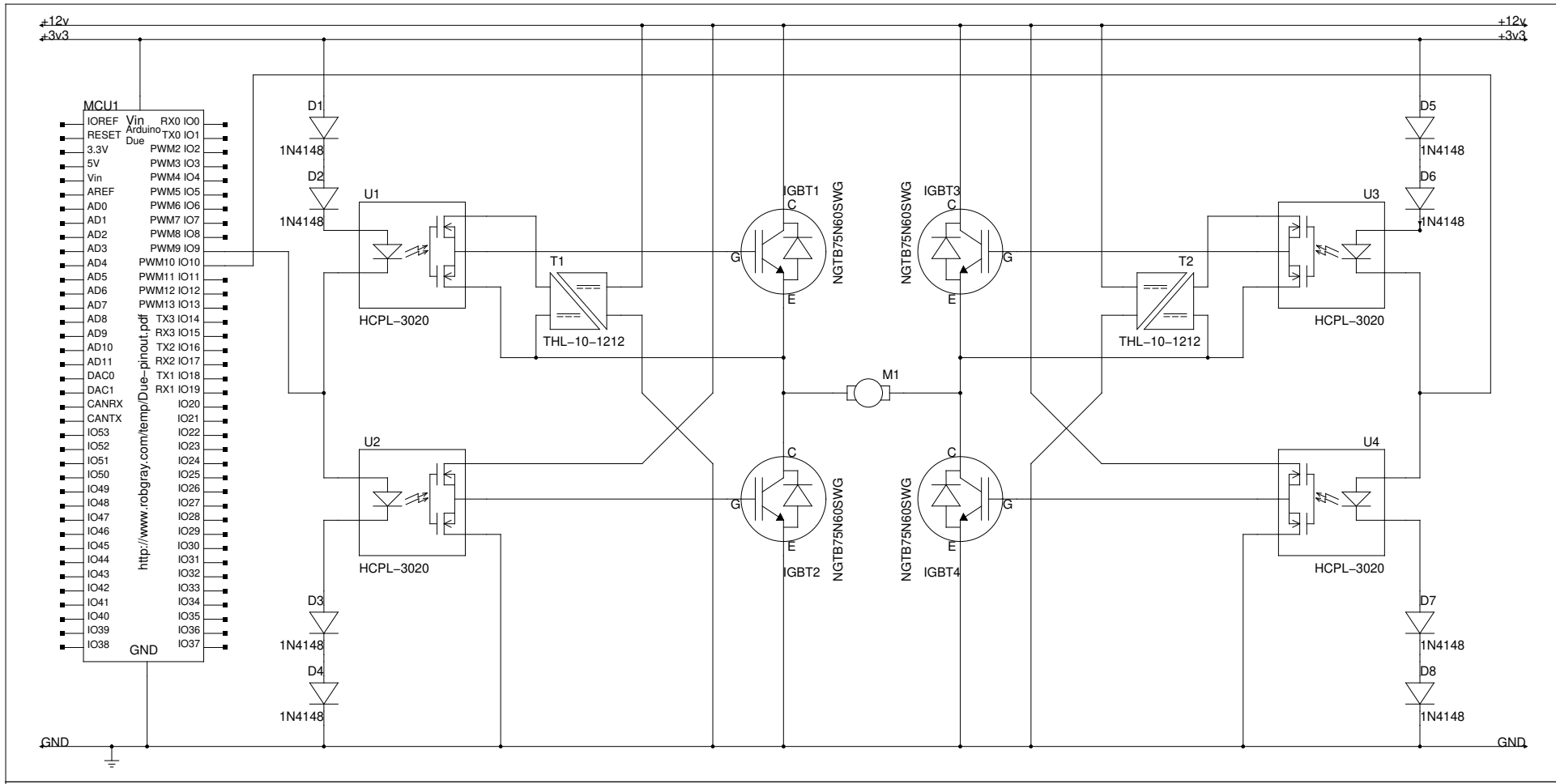
TITLE: Steering Full H-bridge AUTHOR: Graham North CREATED: 21-July-2020
