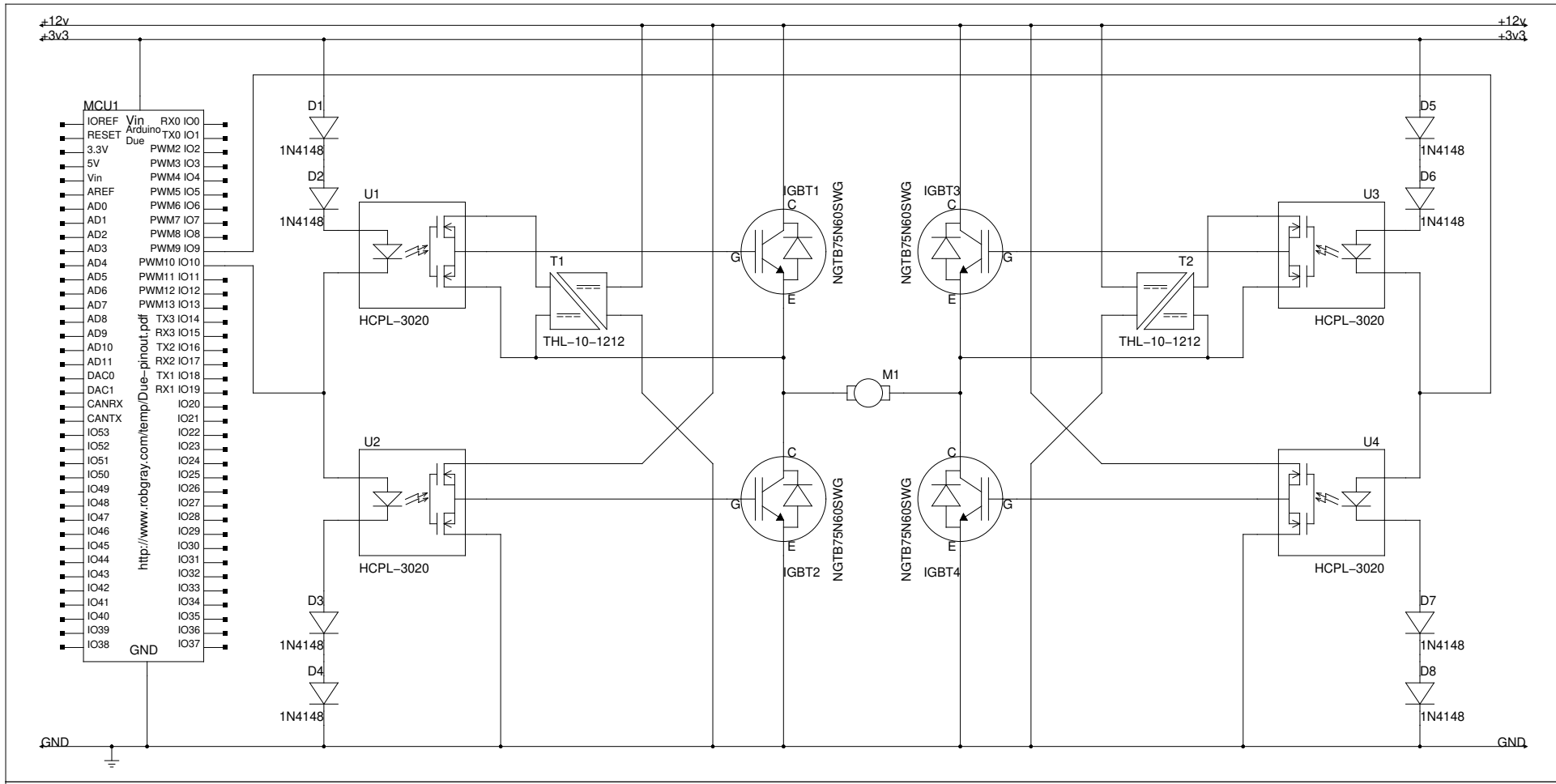
TITLE: Steering H-bridge AUTHOR: Graham North CREATED: 31-July-2020
